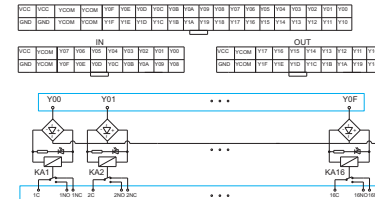
DM108-RM-16-PN-2-4M-100Z(H)
