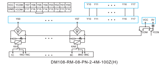
DM108-RM-08-PN-2-4M-100Z(H)
