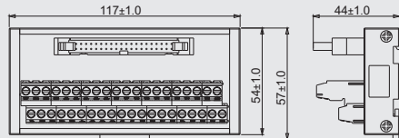
DM50-IDC-40-40-4Y-10Z(H)
