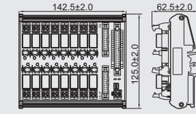
DM108-RMS-16-PN-1-4M-00Z(H)
