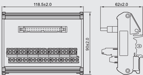
DM72-IDC-40-40-4Y-00Z(H)
