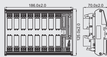
DM108-RM-32-PN-2-4M-100Z(H)
