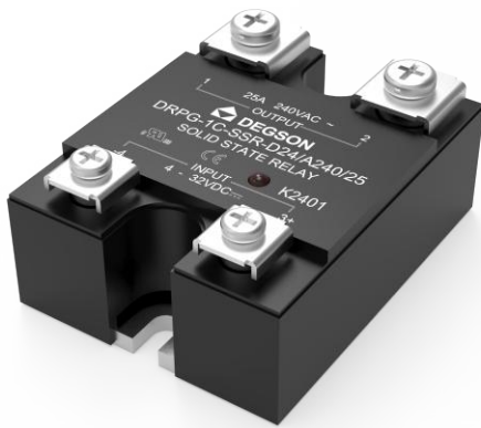
DRPG-1C-SSR-DXX/AXX/X
