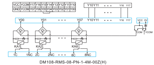
DM108-RMS-08-PN-1-4M-00Z(H)
